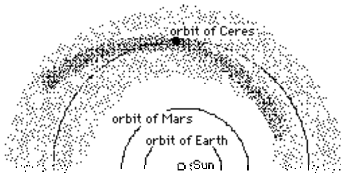
Ceres’ orbit within the main Asteroid Belt and the swath, in relationship to Ceres’ position, in which we’ll find asteroids that will orbit in formation with Ceres for many decades.
